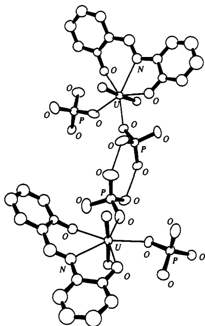
Figure 4. Crystal structure of the complex 19a ·2H 2 PO 4 - . The structure shown contains a crystallographic center of symmetry. Tetrabutylammonium fragments and solvent molecule are omitted for clarity.
