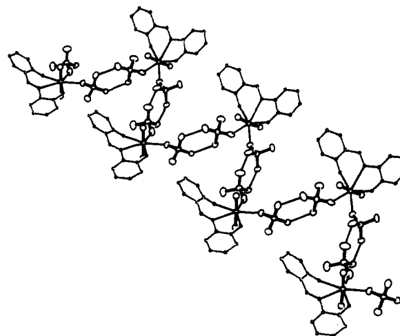
Figure 5. View of the H-bonded ribbon of the complex 19a ·2H 2 PO 4 - .
