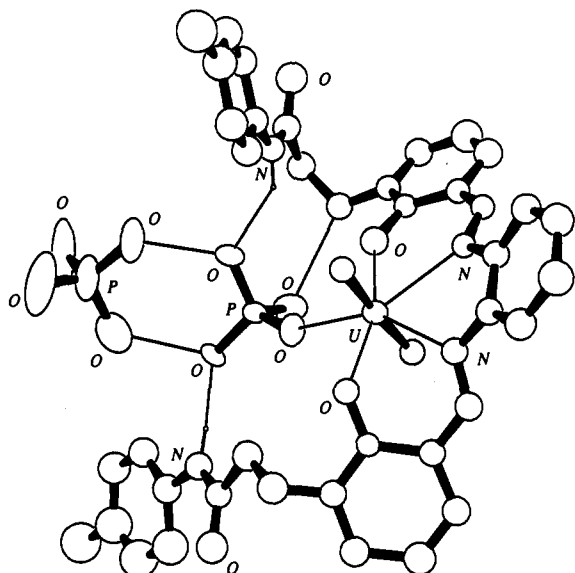
Figure 3. Crystal structure of the complex 14e · 2\text{H}_2\text{PO}_4^- . Tetrabutylammonium fragments and solvent molecules are omitted for clarity.
